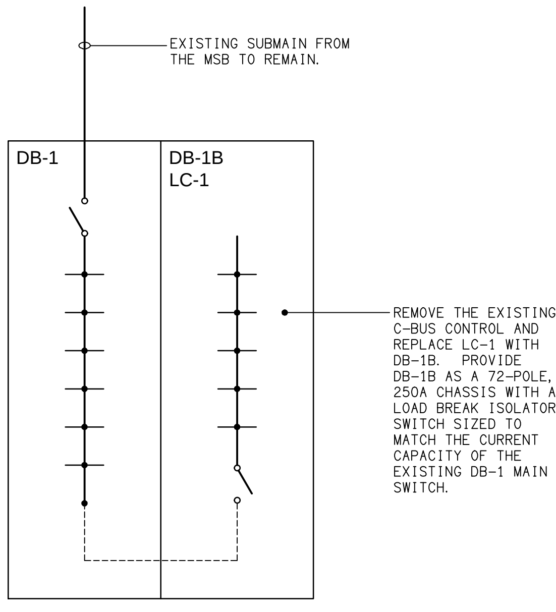
DETAIL DB-1 / LC-1 / DB-1B ELEVATION NOT TO SCALE
